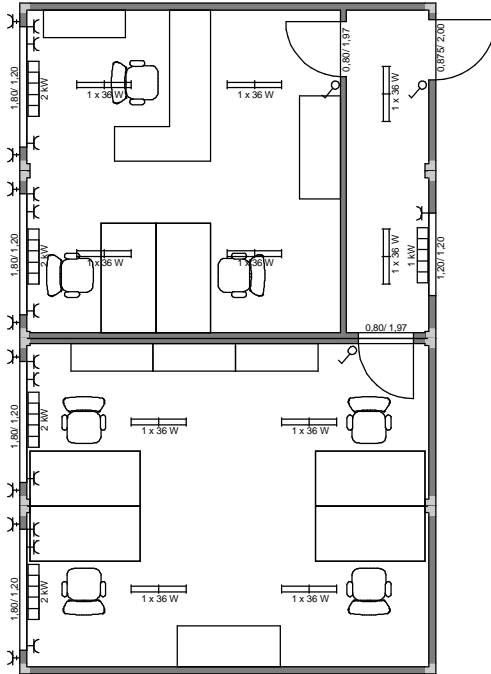
ARS V1 - (LxB) 6,058m x 9,75m; RH = 2,50m
