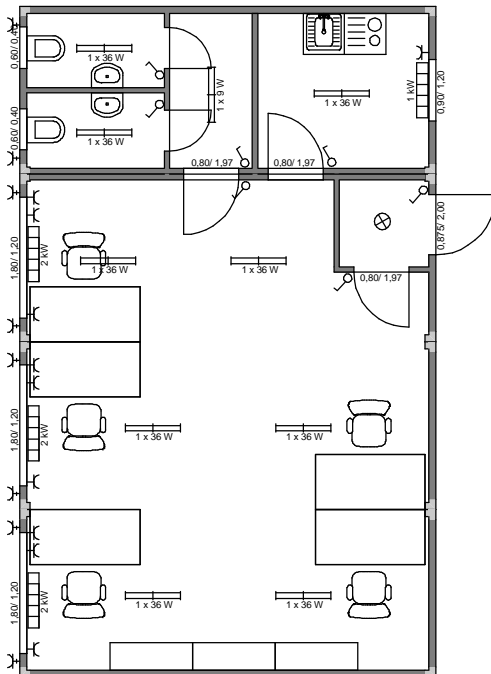
ARS V3 - (LxB) 6,058m x 9,75m; RH = 2,50m
