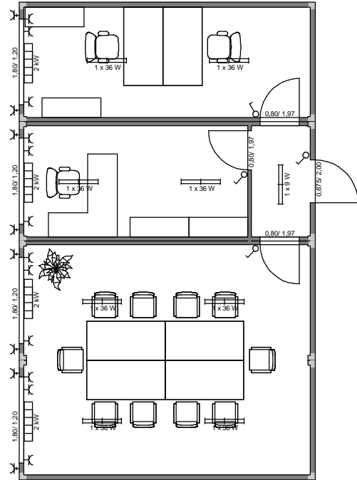
ARS V2 - (LxB) 6,058m x 9,75m; RH = 2,50m
