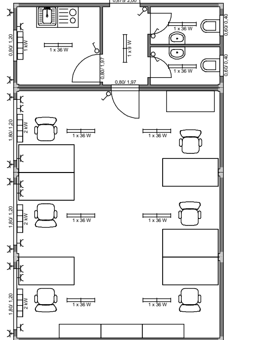
ARS V4 - (LxB) 6,058m x 9,75m; RH = 2,50m
