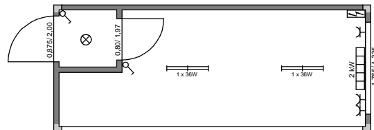
ARS E 6 - (LxB) 6,058m x 2,438m; RH = 2,50m
