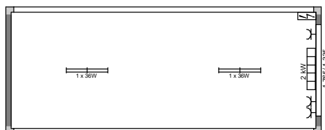
ARS E 9 - (LxB) 6,058m x 2,438m; RH = 2,50m
