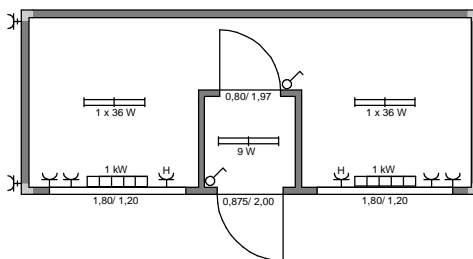
ARS B5 - 6,058m x 2,435m x RH 2,50m
