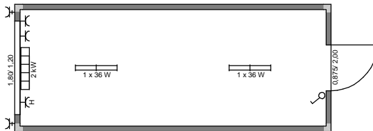
ARS B3 - 6,058m x 2,435m x RH 2,50m
