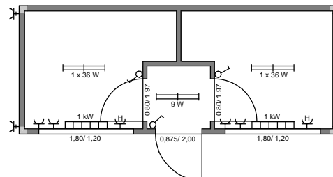
ARS B4 - 6,058m x 2,435m x RH 2,50m
