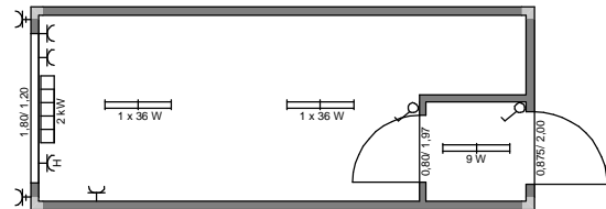
ARS B4 - 6,058m x 2,435m x RH 2,50m
